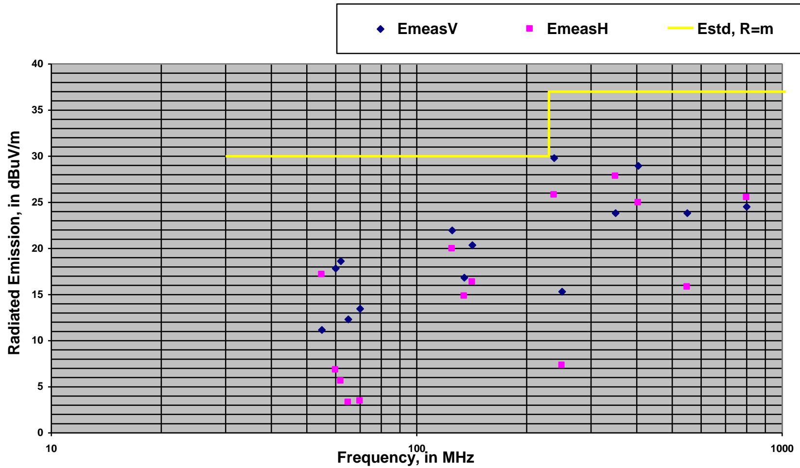
Radiated Emission vrs. EN55022 Class B Standard, Vertical/Horizontal Polarization
